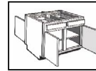
BI_30 30"W X 34 1/2"H X 24"D BI_36 36"W X 34 1/2"H X 24"D BI_42 42"W X 34 1/2"H X 24"D • Two functioning drawers • Four doors • One fixed shelf
