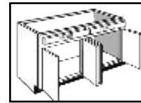
V_48 48"W X 30"H X 21"D V_54 54"W X 30"H X 21"D V_60 60"W X 30"H X 21"D
