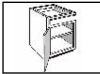
B_12 12"W X 34 1/2"H X 24"D B_15 15"W X 34 1/2"H X 24"D B_18 18"W X 34 1/2"H X 24"D B_21 21"W X 34 1/2"H X 24"D • One fixed half-shelf
