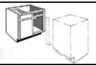
BL_27 27"W X 34 1/2"H X 24"D BL_30 30"W X 34 1/2"H X 24"D BL_33 33"W X 34 1/2"H X 24"D BL_36 36"W X 34 1/2"H X 24"D BL_42 42"W X 34 1/2"H X 24"D BL_48 48"W X 34 1/2"H X 24"D • Blind is 18" Center Stile is 5" • Order BR for blind right or BL for blind left. ( Illustration is blind right) • Order 3" - 6" smaller than wall space
