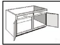
B_27SB 27"W X 34 1/2"H X 24"D B_30SB 30"W X 34 1/2"H X 24"D B_33SB 33"W X 34 1/2"H X 24"D B_36SB 36"W X 34 1/2"H X 24"D B_42SB 42"W X 34 1/2"H X 24"D • No interior shelves
