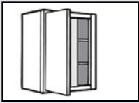
WBL_2430 24"W X 30"H X 12"D WBL_3030 30"W X 30"H X 12"D • Blind is 12" • Order .BR for blind right or .BL for blind left. ( Illustration is blind right) • Order 3" - 6" smaller than wall space • Center Stile is 5" • Two adjustable shelves
