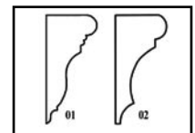
Crown 01: 2 3/4"H X 1 3/8"TH X 72"L Crown 02 2 3/4"H X 1 3/8"TH X 72"L
