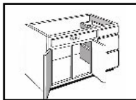
V_42E 42"W X 30"H X 21"D V_48E 48"W X 30"H X 21"D V_54E 54"W X 30"H X 21"D V_60E 60"W X 30"H X 21"D • Order .DR for drawers right or .DL for drawers left • One 3 1/4"H & Two 5"H drawers
