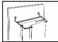
.TR 12 5/8"W X 6 1/2"D Add .TR to the end of cabinet model numbers to include towel rack. On cabinets with more than one door, please specify which door.
