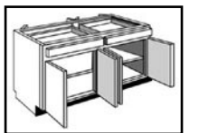
B_48 48"W X 34 1/2"H X 24"D • Two functioning drawers • Eight doors • One fixed shelf
